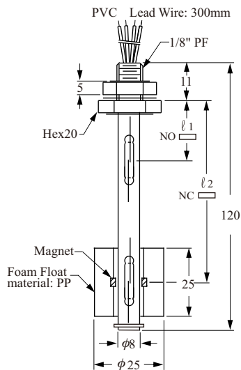
O-Ring: VITON
